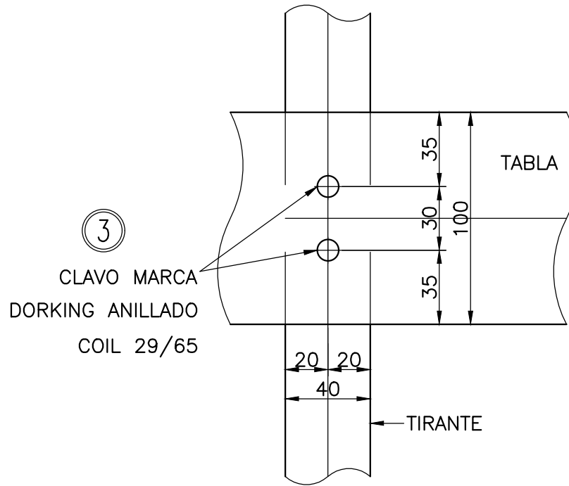
UNION C1 ESC. 1:2.5 CANT: 2
